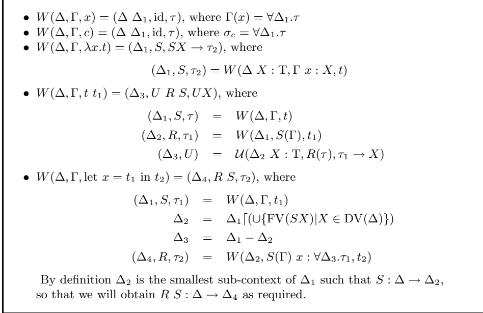
Fig. 4. Algorithm W
