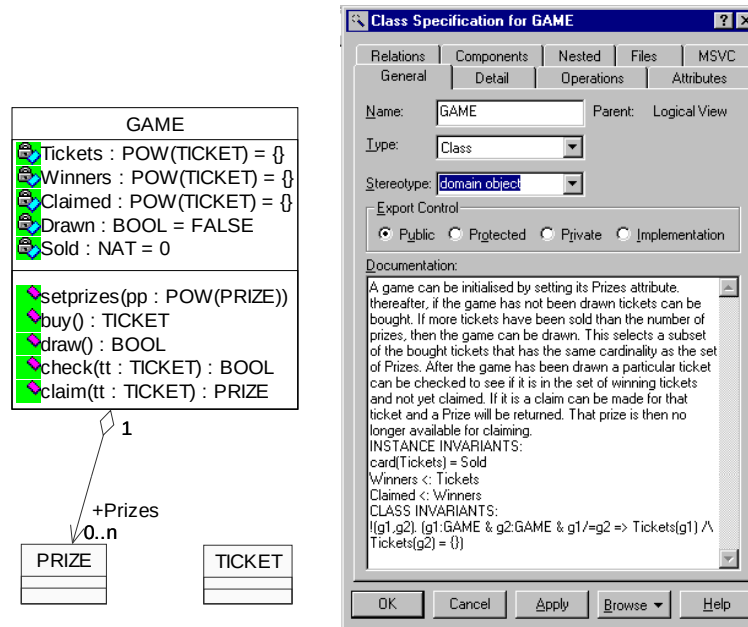
Fig. 1. Example Class Diagram and Class Specification
